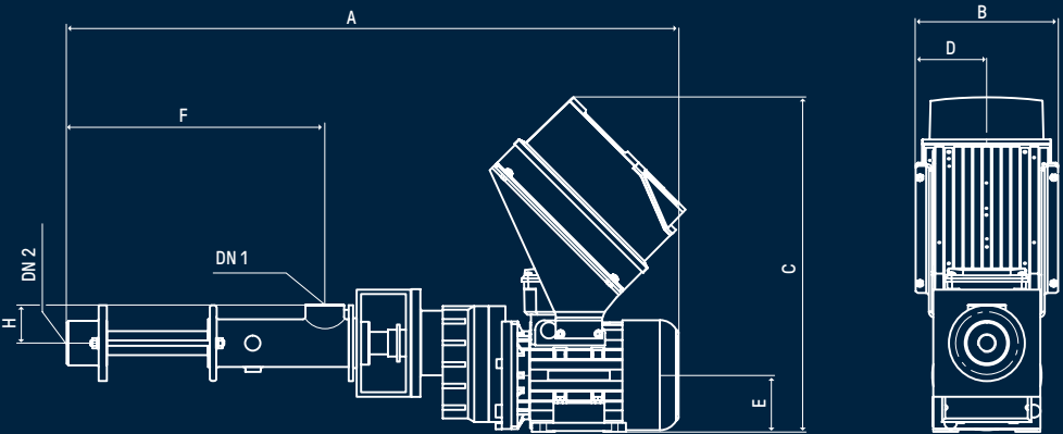
MD – Intelligent Metering Pump
